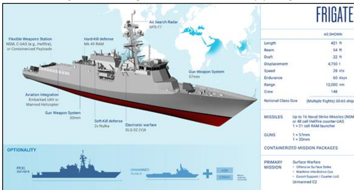
Figure 6. Rendering and Selected Details of FF(X) Design
