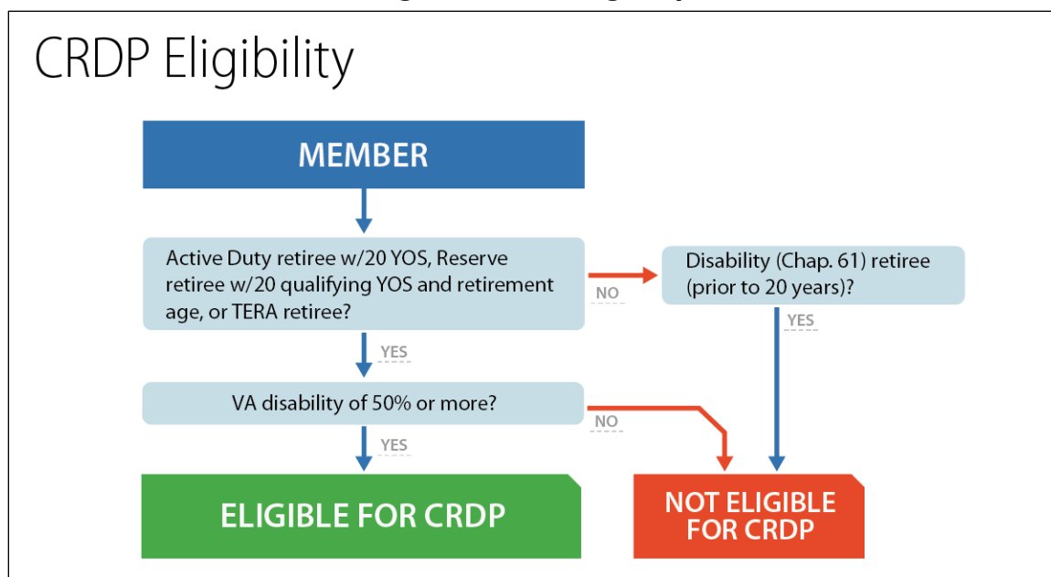
Figure 4. CRDP Eligibility
