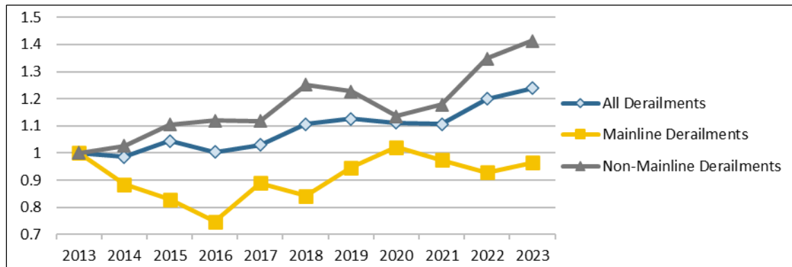
Figure 4. Change in Derailment Rate per Train-Mile by Track Type, CY2013-CY2023 (Index) I = 2013 value
