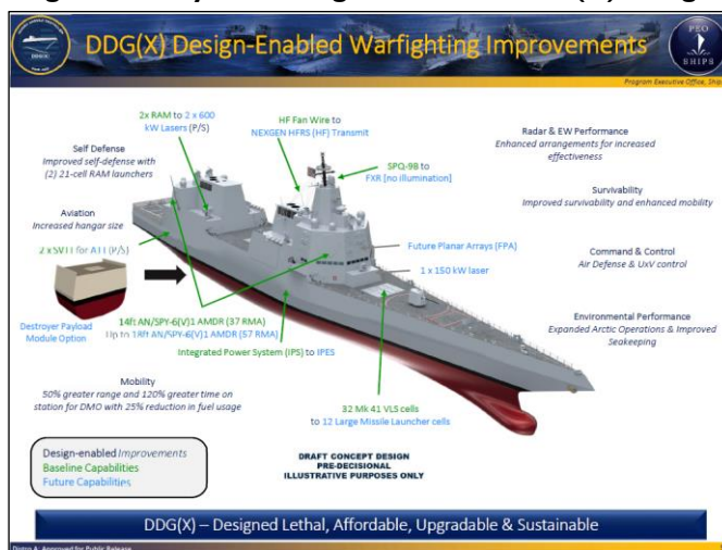
Figure 1. Navy Rendering of Notional DDG(X) Design
