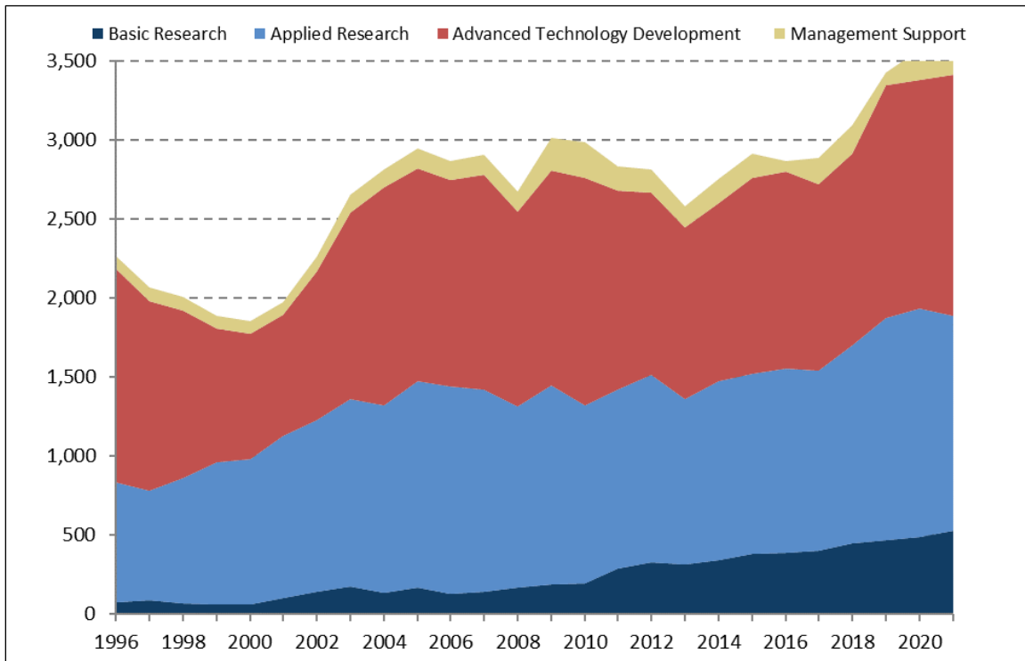
Figure 2. DARPA Funding by Character of Work, FY1996-FY2021
