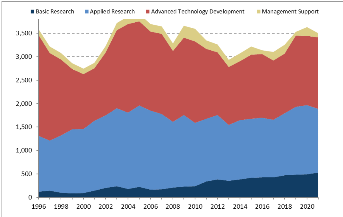
Figure 3. DARPA Funding by Character of Work, FY1996-FY2021
