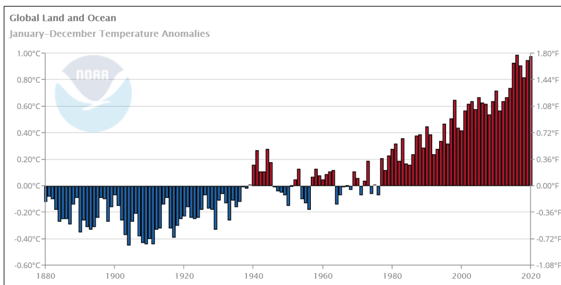
Figure 1. Anomalies of Global Average Surface Temperature, 1880-2020 (in degrees Celsius and Fahrenheit)
