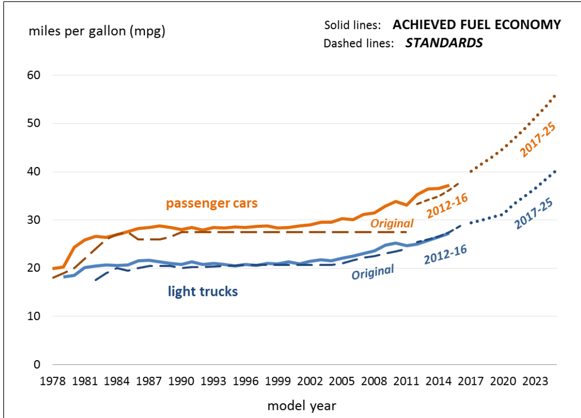
Figure I. CAFE Standards and Achieved Fuel Economy, MYs 1978-2025
