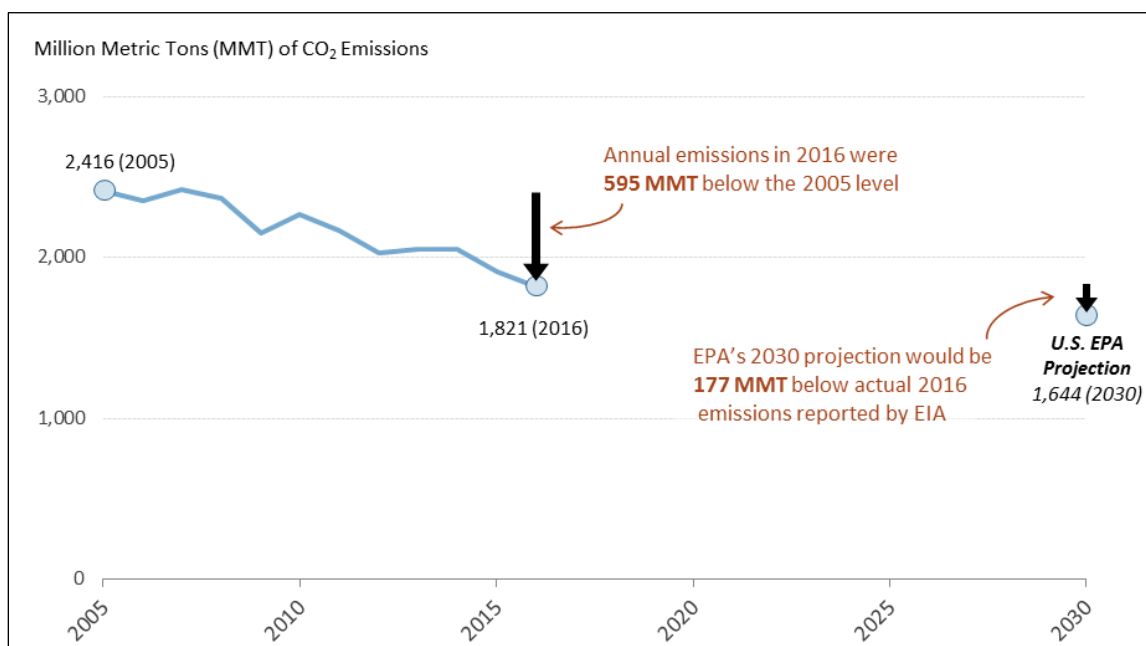
Figure 1. GHG Emissions from Electric Power Generation, 2005-2016
