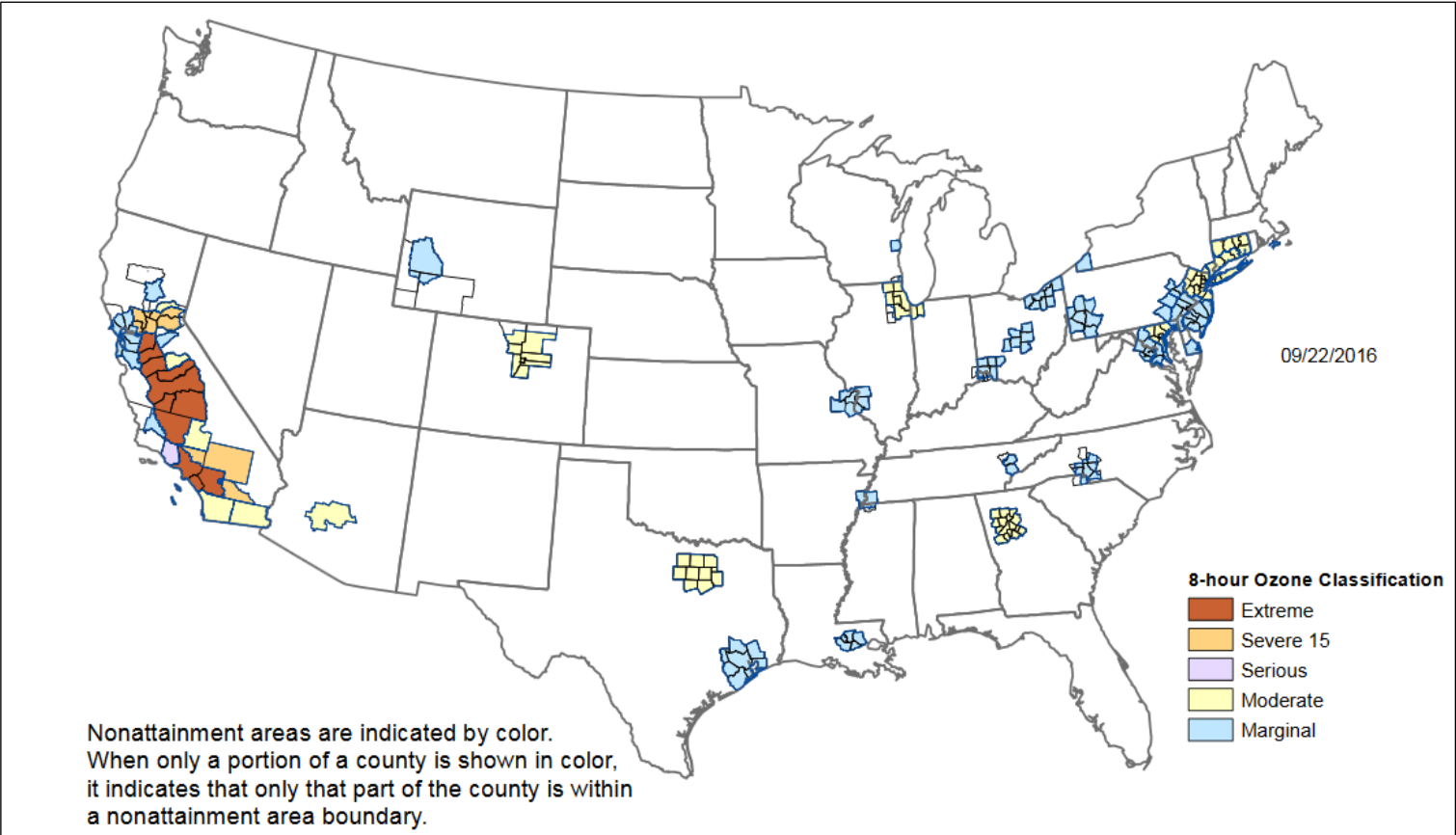
Figure 1. Current Ozone Nonattainment Areas, September 2016 (2008 Standard, 0.075 ppm)
