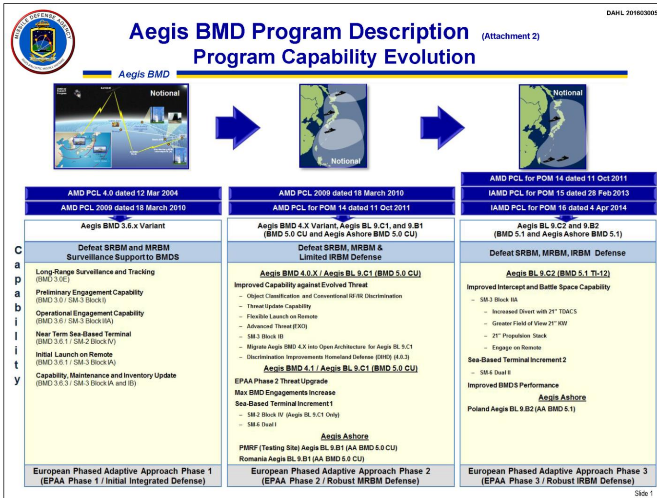
Figure 1. Aegis BMD System Variants (Summary of capabilities)
