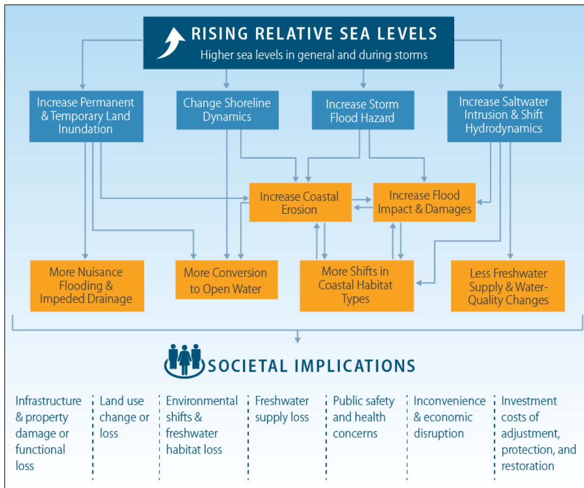
Figure 7. Selected Coastal Effects of Relative Sea-Level Rise
