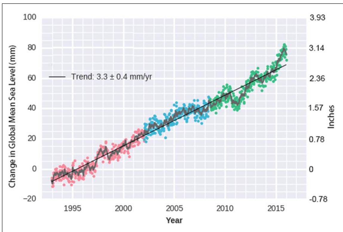
Figure 1. Global Sea-Level Rise from Satellite Measurements
