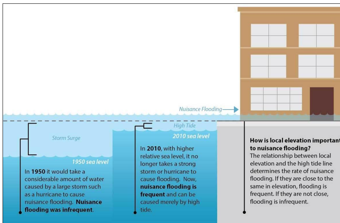
Figure 11. Illustration of Increase in Coastal Nuisance Flood Hazard
