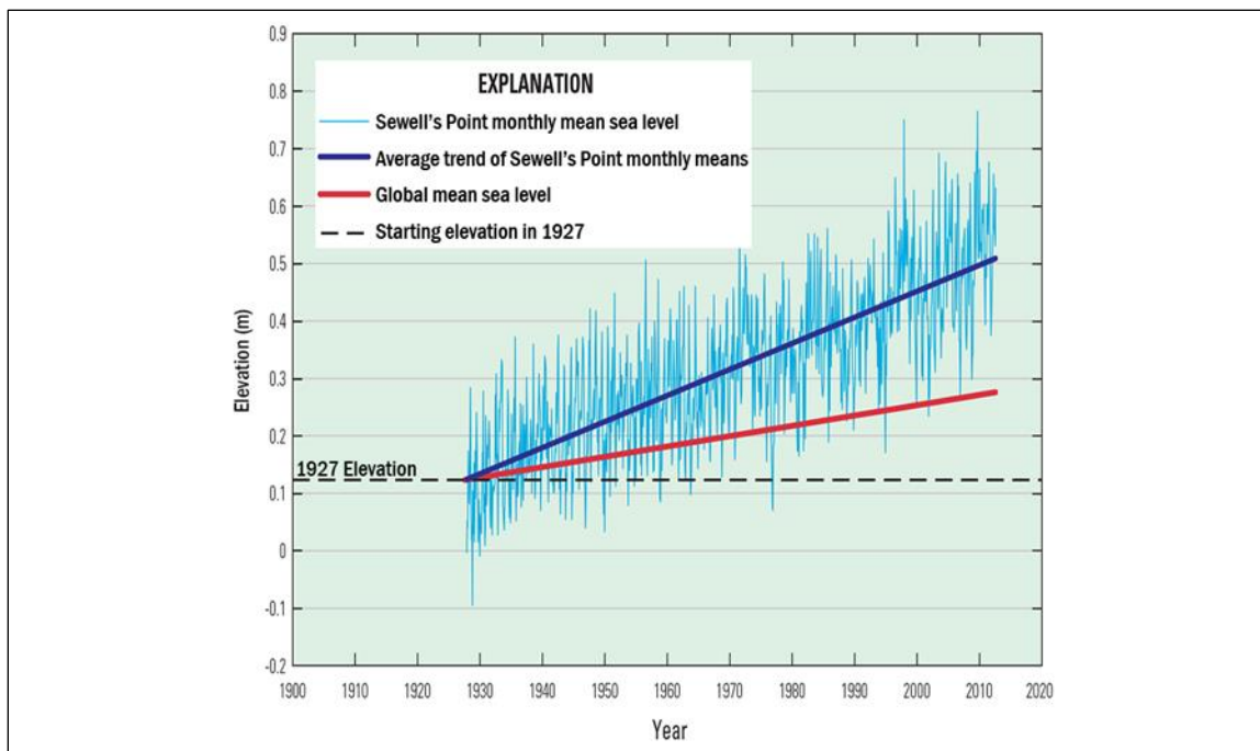
Figure 6. Monthly Average Sea-Level Elevation at Sewell's Point, Norfolk, VA
