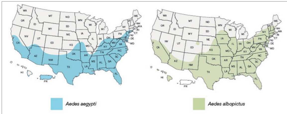
Figure 2. Estimated Range of Aedes Mosquito in the United States
