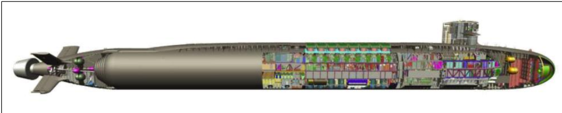
Figure 2. Ohio Replacement Boat Notional cutaway illustration
