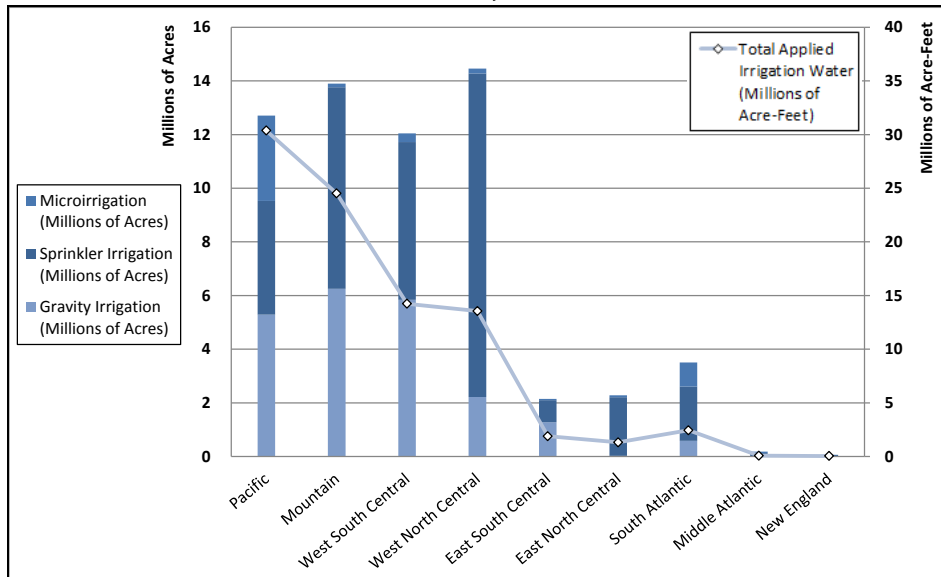
Figure 5. Irrigation Technologies by Acres and Applied Water by Acre-Feet by Census Division, 2013
