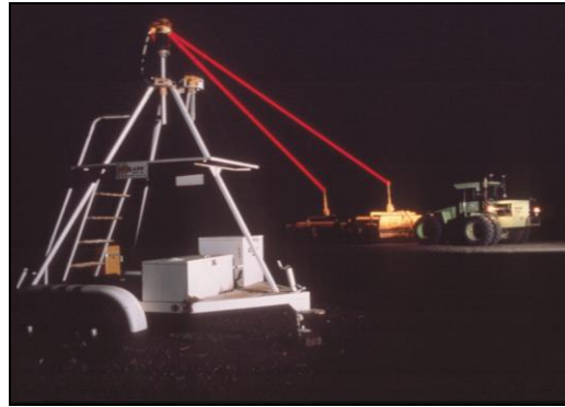
Figure 10. Laser-Leveling Irrigation Land
