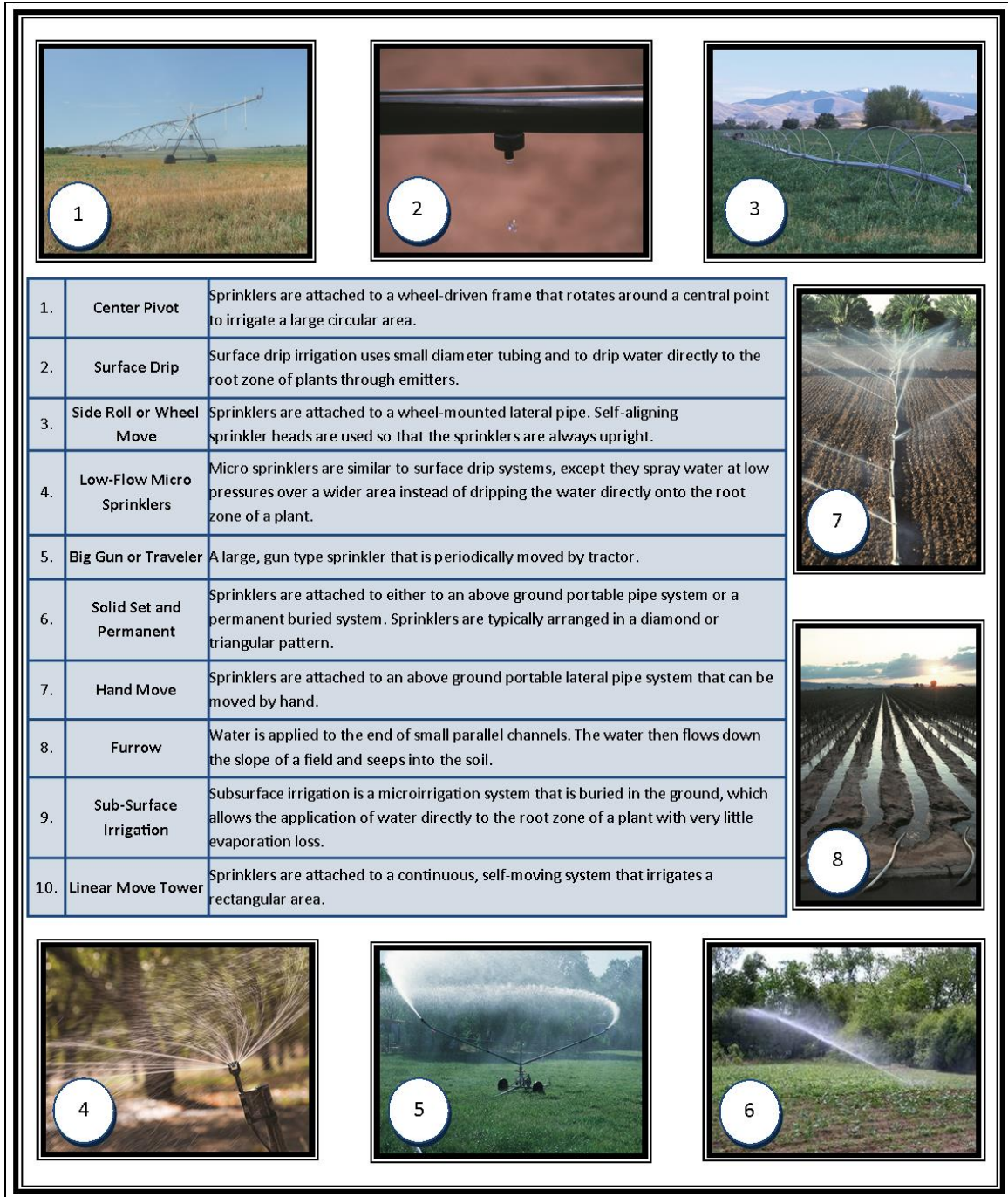
Figure 12. Common Irrigation Technologies in the United States
