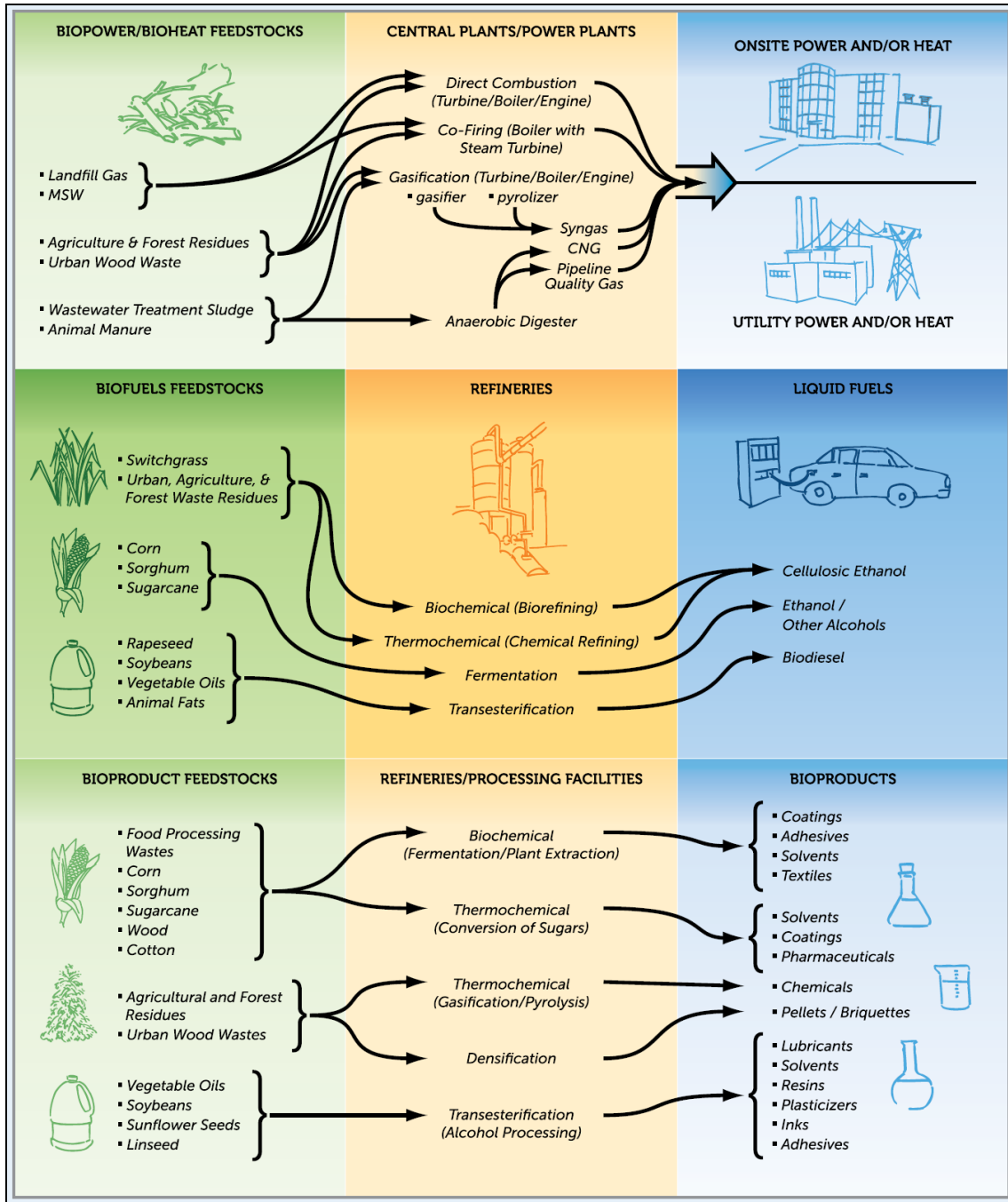
Figure 1. Bioenergy and Bioproduct Conversion Processes
