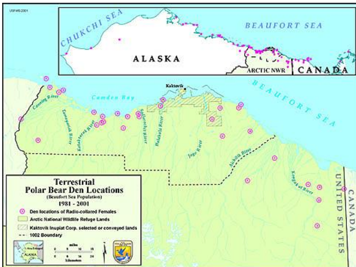
Figure 7. Terrestrial Polar Bear Den Locations (1981-2001)
