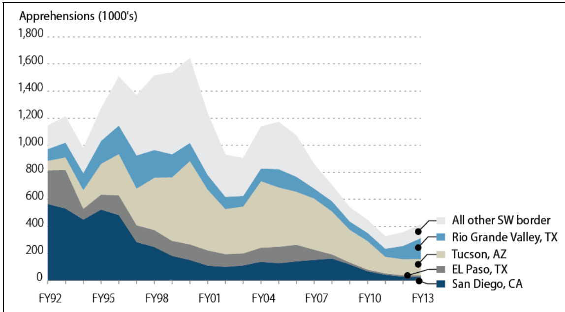
Figure 6. U.S. Border Patrol Apprehensions of Deportable Aliens, Southwest Border, by Selected Sectors, FY1992-FY2013
