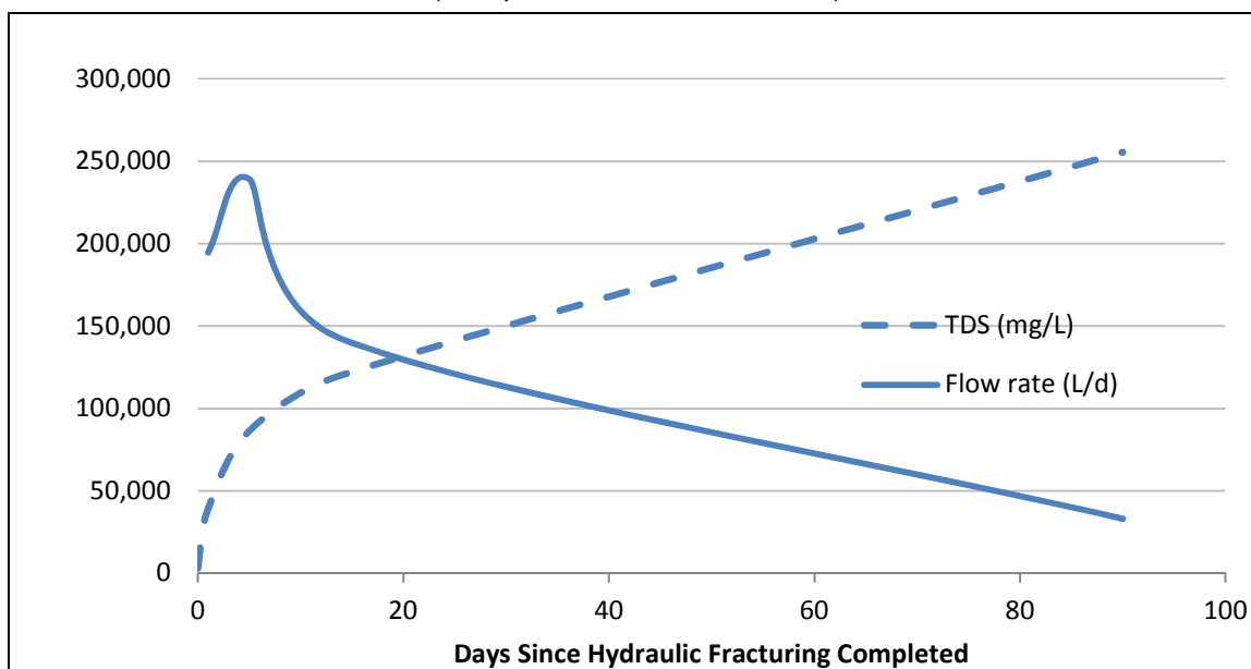
Figure 7. Change in the Total Dissolved Solids Concentration of Produced Fluids over Time
