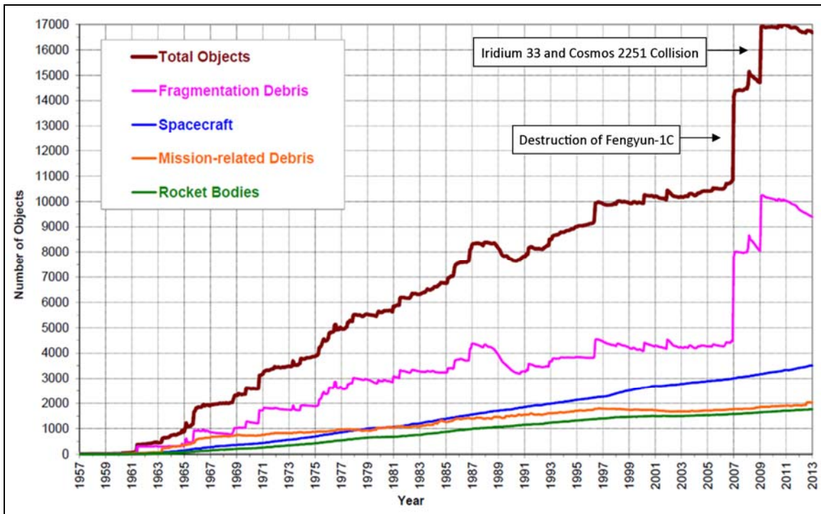
Figure 1. Monthly Number of Objects in Earth Orbit by Object Type
