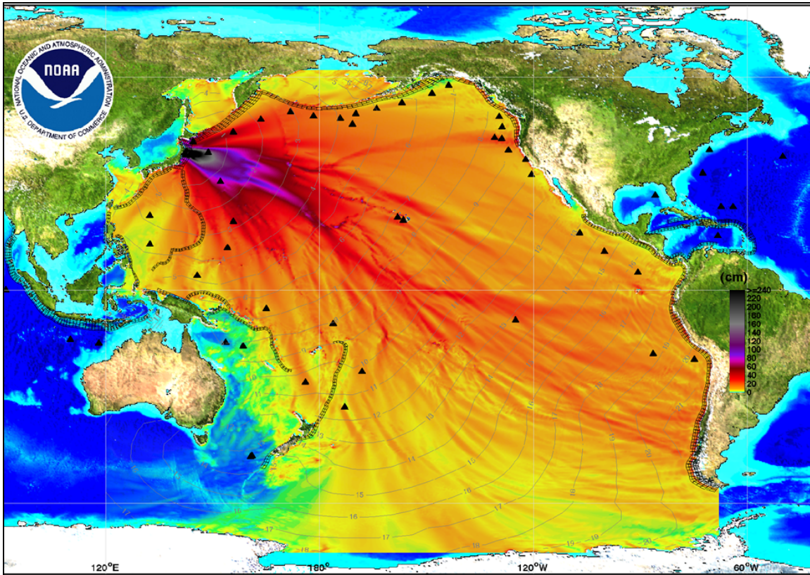
Figure I. Results from NOAA Model Depicting the March 11, 2011 Tsunami Propagating Across the Pacific Ocean
