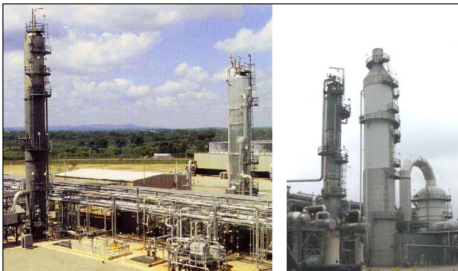
Figure 14. Amine-Based Post-Combustion CO 2 Capture Systems Treating a Portion of the Flue Gas from a Coal-Fired Power Plant in Oklahoma, USA (left), and a Natural Gas Combined Cycle (NGCC) Plant in Massachusetts, USA (right)
