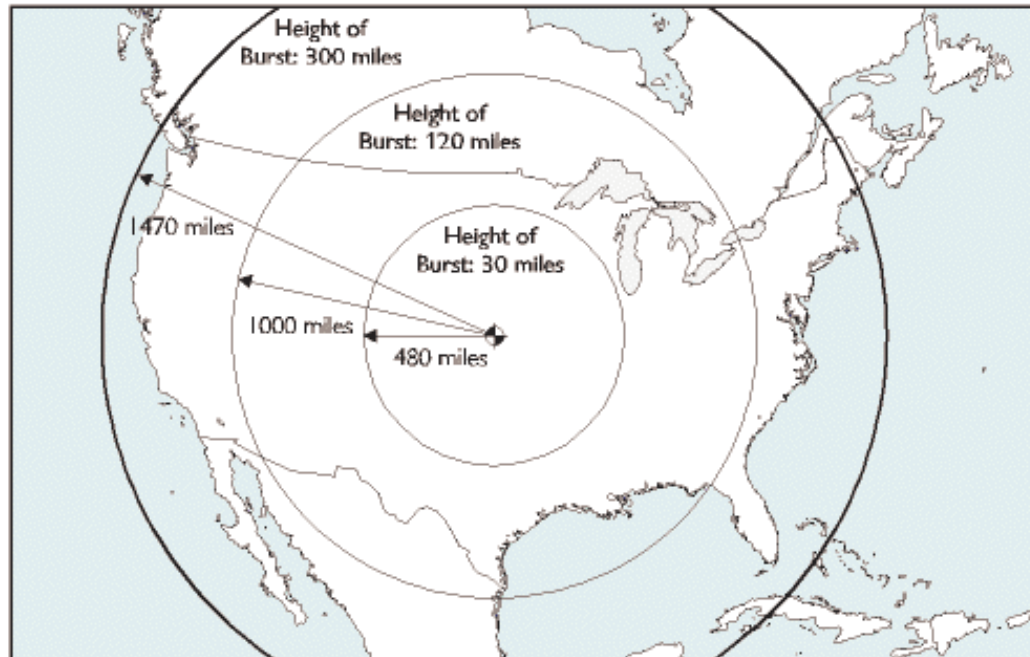
Figure 1. Estimated Area Affected by High-Altitude EMP
