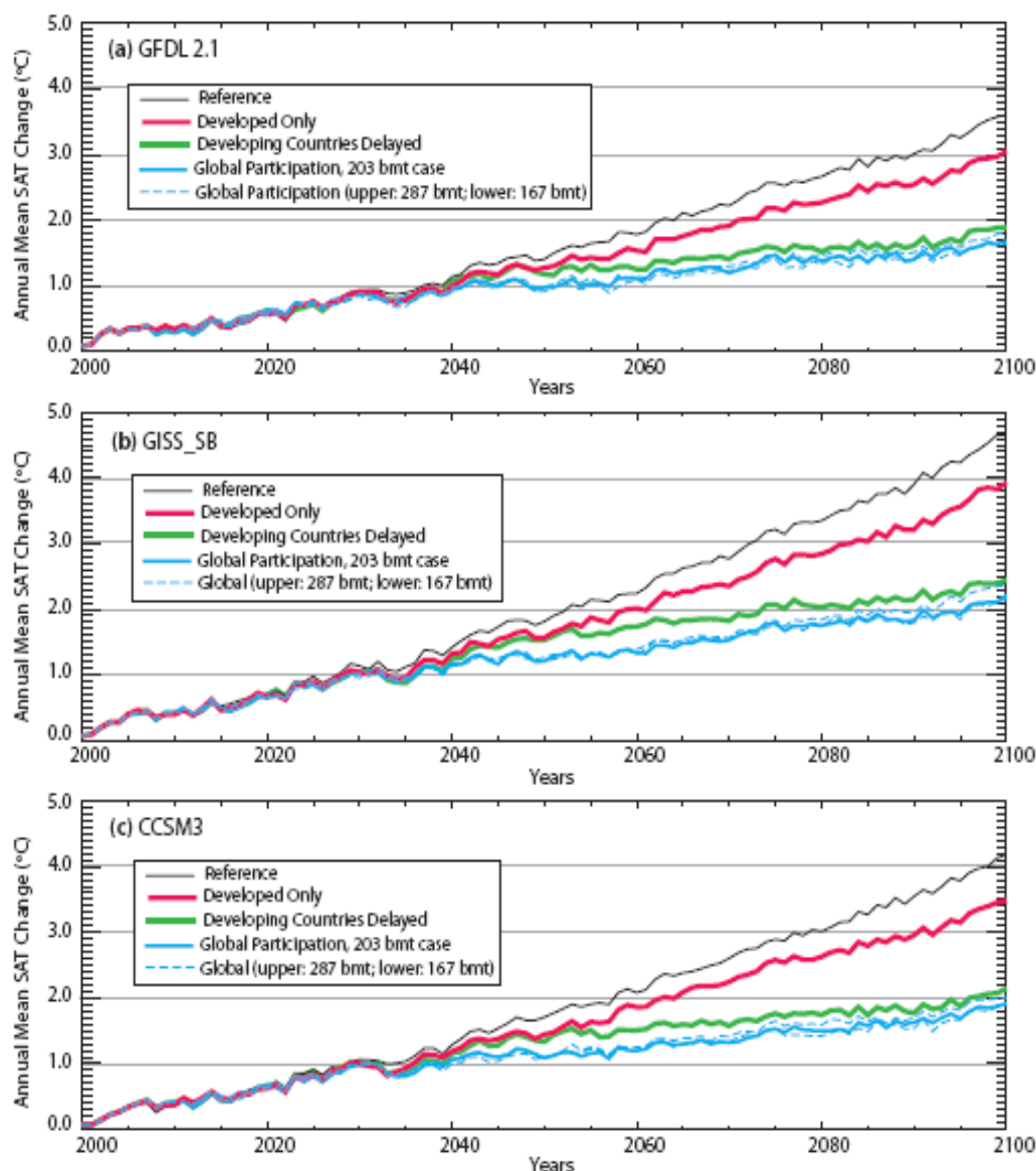
Figure 11. Global Mean Surface Air-Temperature Increase in Six Scenarios Using the MIT IGSM
