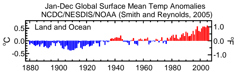
Figure 1. Global Temperature Change Since the Industrial Revolution
