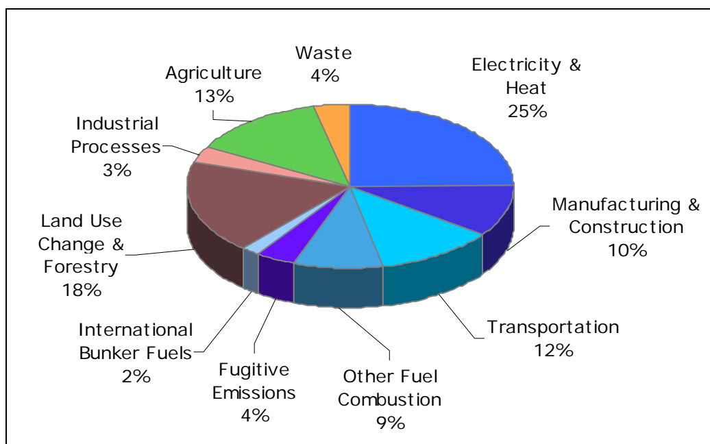
Figure 4. Sectoral Shares of Global GHG Emissions in 2000
