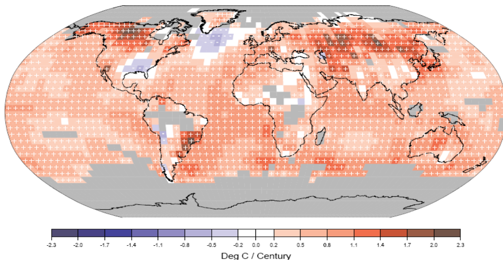
Figure 2. Trends in Average Annual Temperature, 1901-2005
