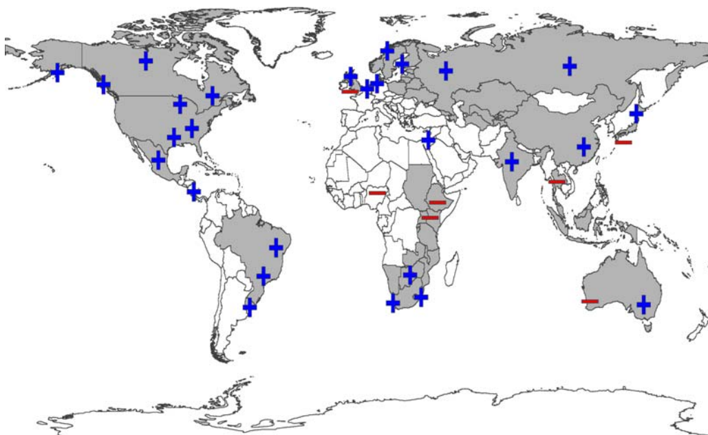
Figure 3. Changes in Frequency of Extreme Precipitation
