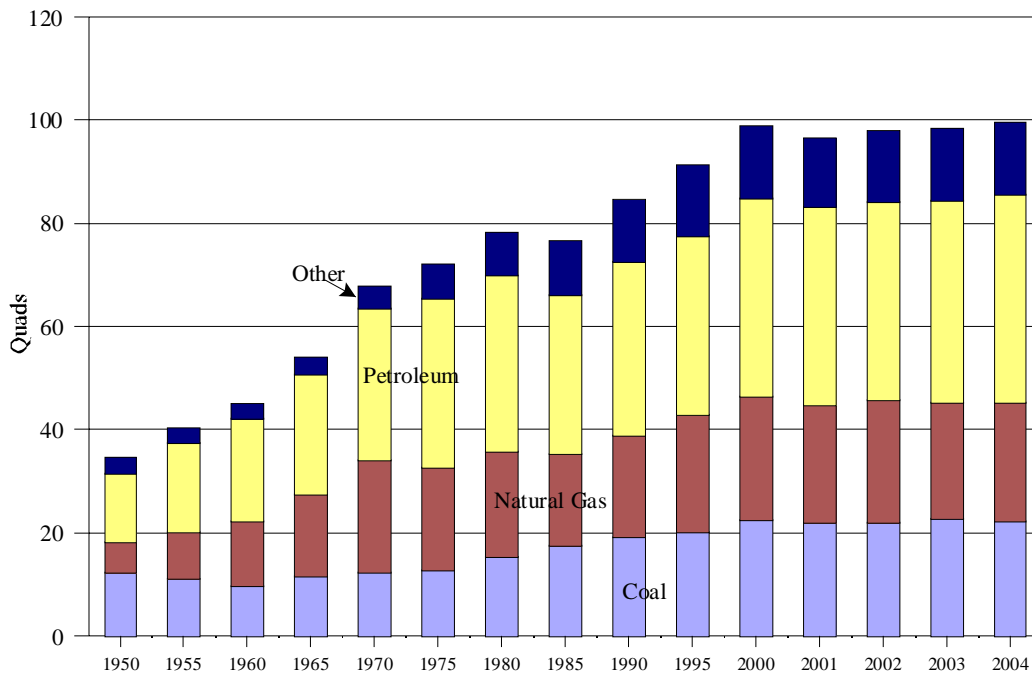
Figure 3. Energy Consumption, 1950-2004
