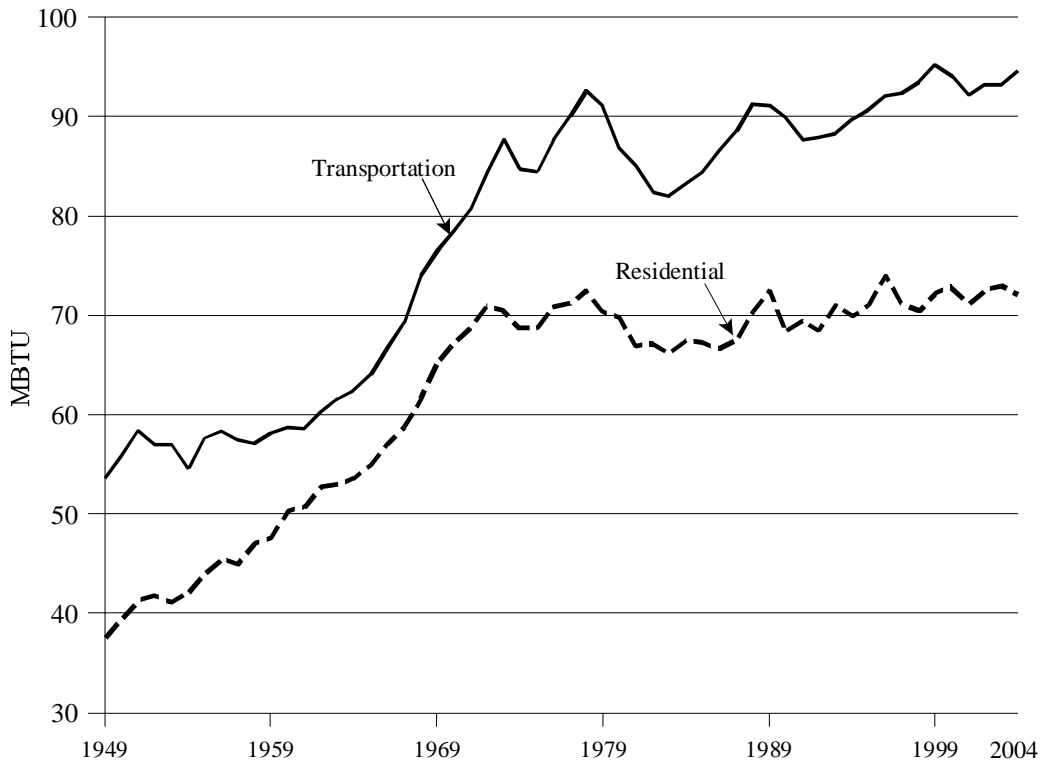
Figure 1. Per Capita Energy Consumption in Transportation and Residential Sectors, 1949-2004
