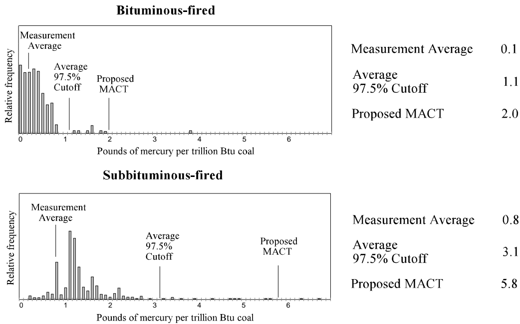
Figure 1. Effect of Statistical Treatment on Proposed MACT Standard for Bituminous- and Subbituminous-fired Facilities
